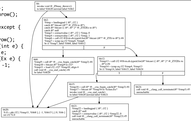
CFG for '_Z1fv' function
