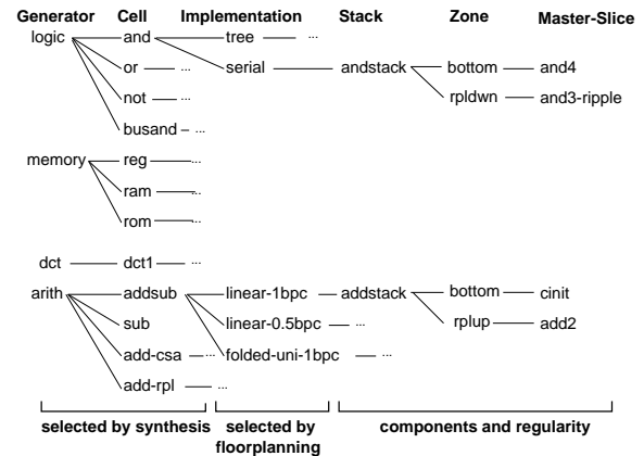
Figure 2: FLAME design entities
