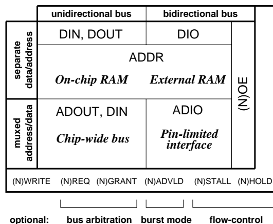
Figure 3: Bus architecture taxonomy
